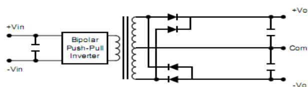
Dual Output
