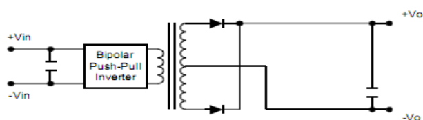
Single Output
